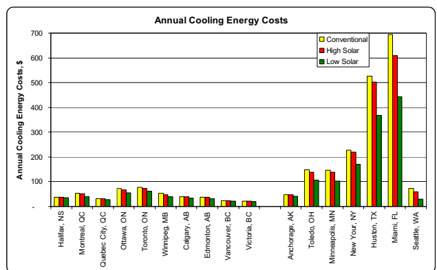
Figure 11 Bar graph showing cooling costs computed for N.A. locations (US locations in US$, Canadian locations in Can$).
