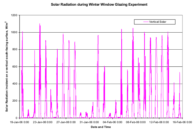
Figure 4 Solar Radiation Incident on a Vertical South-facing surface, during Winter test period
