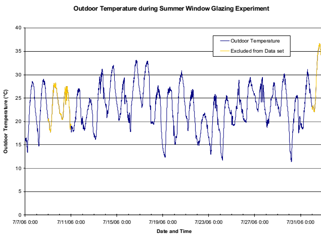
Figure 5 Range of Outdoor Temperatures during Summer test period
