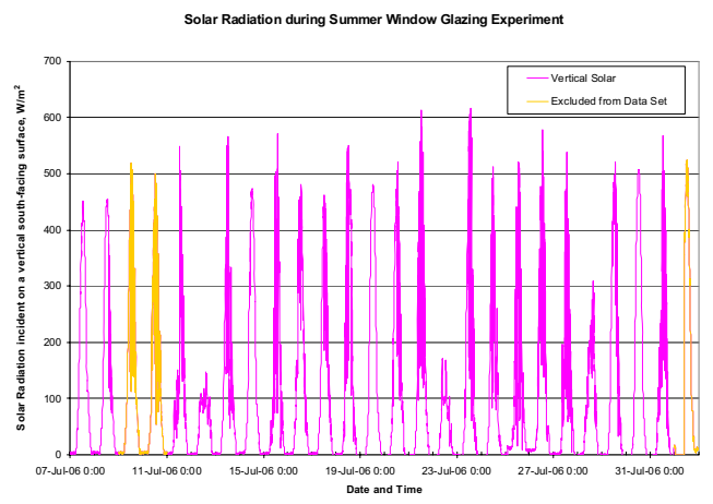
Figure 6 Solar Radiation Incident on a Vertical South-facing surface, during Summer test period
