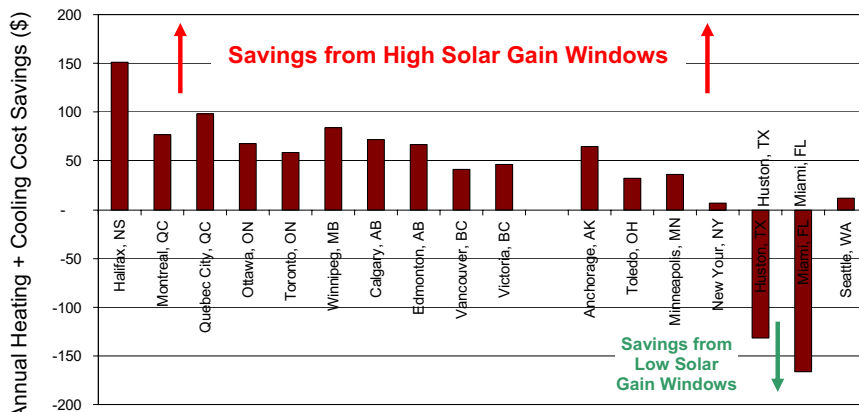
Figure 12 Total annual energy cost differences between high SHGC and low SHGC glazing in different NA locations (US locations in US$. Canadian locations in Can$).
