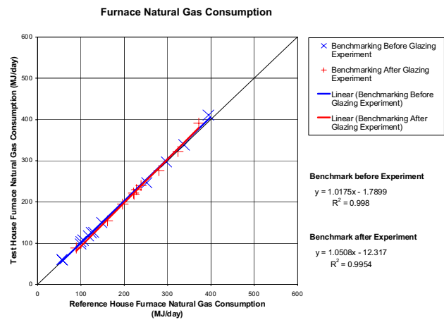
Figure 2 Winter Benchmarking Furnace Gas Consumption Curve before and after the experiment.
