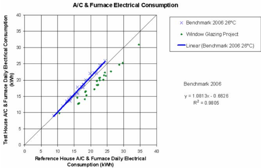
Figure 8 Comparison of the cooling energy consumption of the reference and test houses during summer period.
